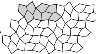
Fig. 1. Convex pentagonal tiles of type 1–10.
