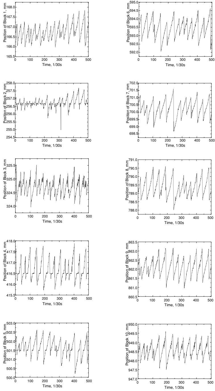
Fig. 3. Variation of position of each block in Case 8.
