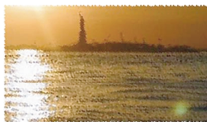
(e) 9973 points
