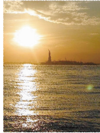
(b) 30000 points
