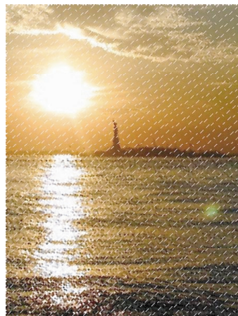
(c) 25637 points
