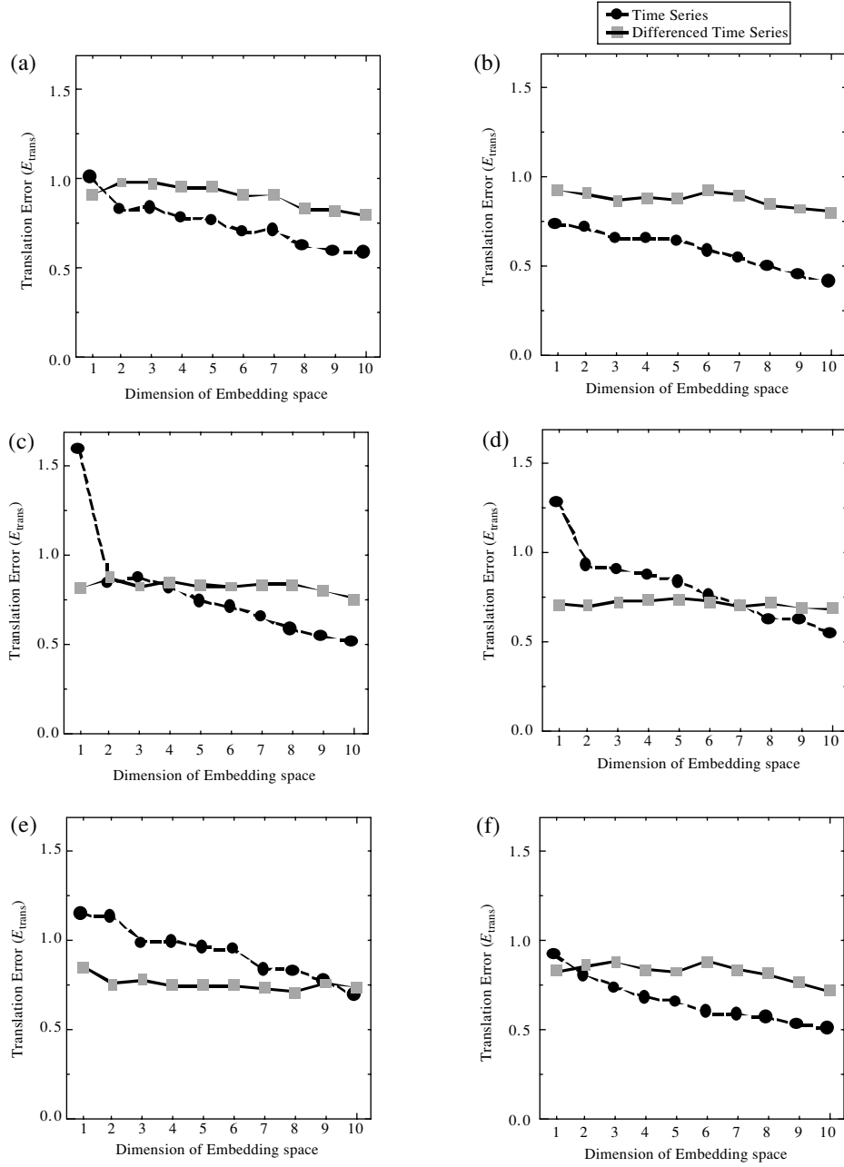
Fig. 3. For each embedding dimension, we calculated the translation errors that were derived from (a) lateral time series when subjects were in the RS, (b) anterior/posterior time series when subjects were in the RS, (c) lateral time series when subjects viewed the display of the previous model, (d) anterior/posterior time series when subjects viewed the display of the previous model, (e) lateral time series when subjects viewed the OCB display, and (f) anterior/posterior time series when subjects viewed the OCB display.
