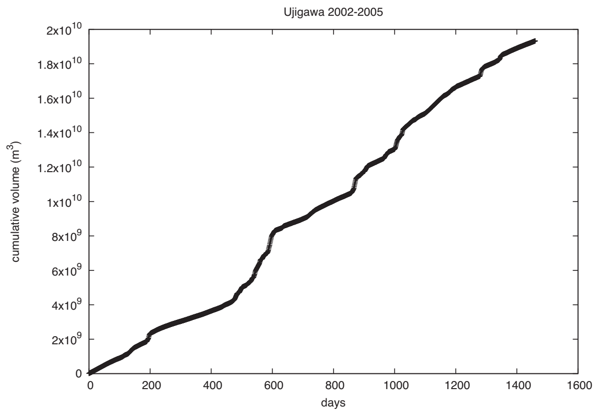
Fig. 2. Cumulative flow volume of Ujigawa (Uji-river) for four years from 2002 to 2005.
