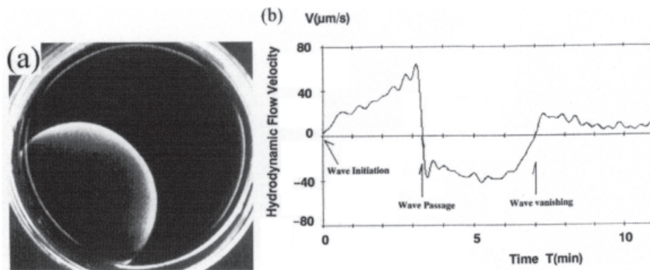
Fig. 4. (a) Excitation of a single chemical wave which propagates with a constant velocity v . The size of the dish is about 6.8 cm. (b) Hydrodynamic flow induced by the single circular wave propagation. The velocity of the flow v_s is measured near the surface of the BZ solution layer. Direction of the flow measured near the surface is reverse to that of the flow measured near the bottom.
