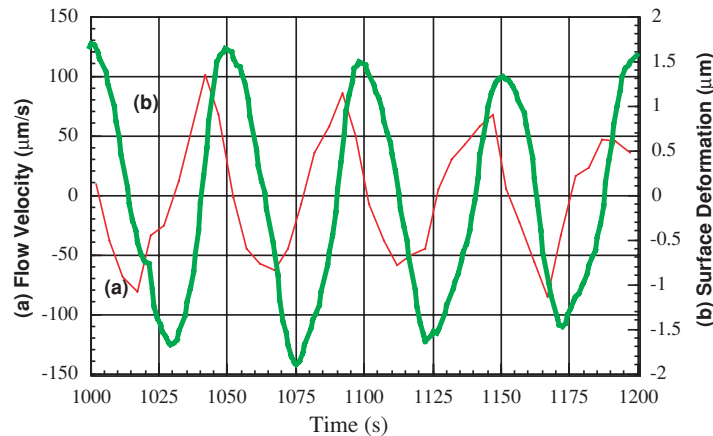
Fig. 11. Comparison between the convection velocity v_x (thin solid line) and the surface deformation h(t) (thick solid line) obtained by Eq. (1) (SAKURAI et al. , 1997a).
