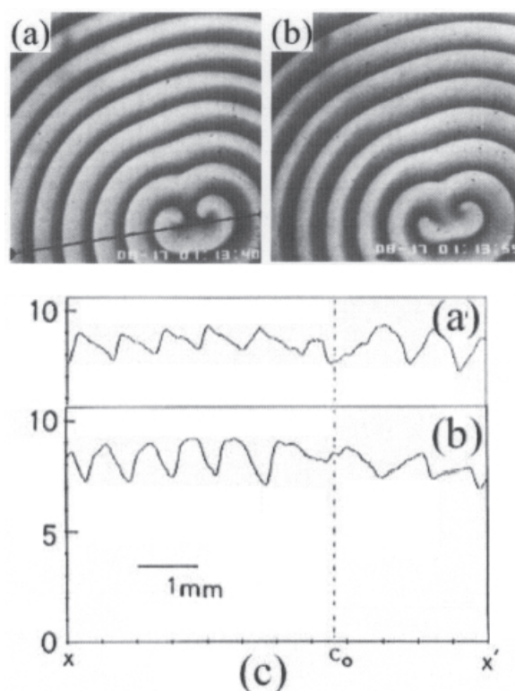
Fig. 8. Deformation of chemical wave profiles by the oscillatory flow (MIIKE and MÜLLER, 1993). Sectional profiles along tilted solid line in (a) are shown in (c). Left half profiles in (c) are with surface flow against (a) and in the direction (b) of wave propagation. On the courtesy of Prof. S. C. Müller.
