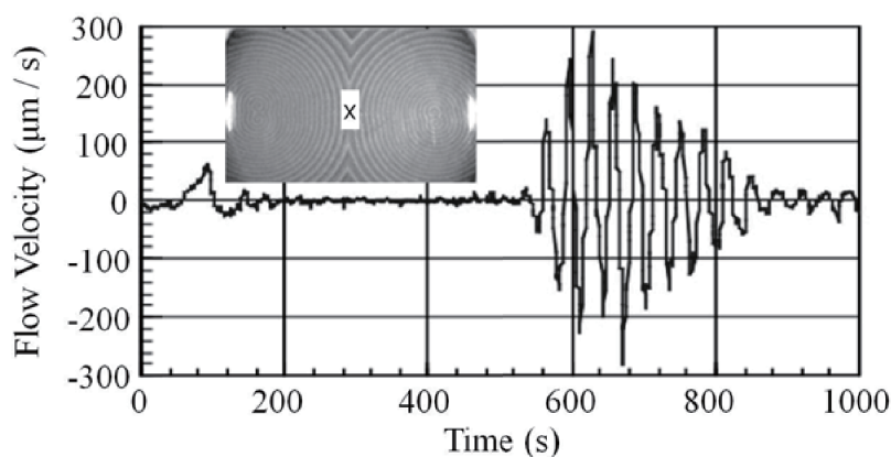
Fig. 16. Temporal evolution of the flow velocity associated with two spiral pairs (TSPs). The flow velocity was measured at the location x in the picture near the surface of a BZ solution layer at the center of the Petri dish (Sakurai et al. , 2004).
