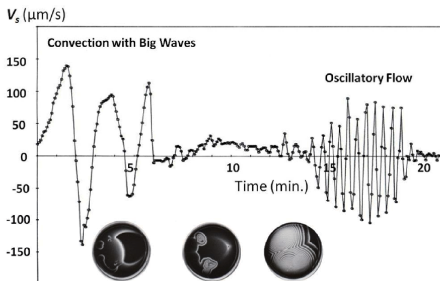
Fig. 25. Convective pattern dynamics caused by a transition from discrete propagation of a chemical wave (like the big wave) to spiral waves (Miike and Sakurai, 2003). The oscillatory flow was induced spontaneously at around t = 14 min after triggering a single chemical wave ( t = 0 ) in a thin solution layer of the BZ-reaction. The pictures at the bottom are the corresponding patterns.
