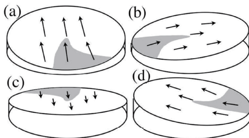
Fig. 24. Schematic presentation of the time evolution of surface flow structure and surface deformation, as observed during the rotating spiral flow developed in a thin solution layer of the BZ-reaction. A chemical spiral core was excited at the middle of the Petri dish (Mahara et al. , 2009). The global structure of surface flows is determined from chemical wave pattern contrast and surface flow direction in Fig. 22.
