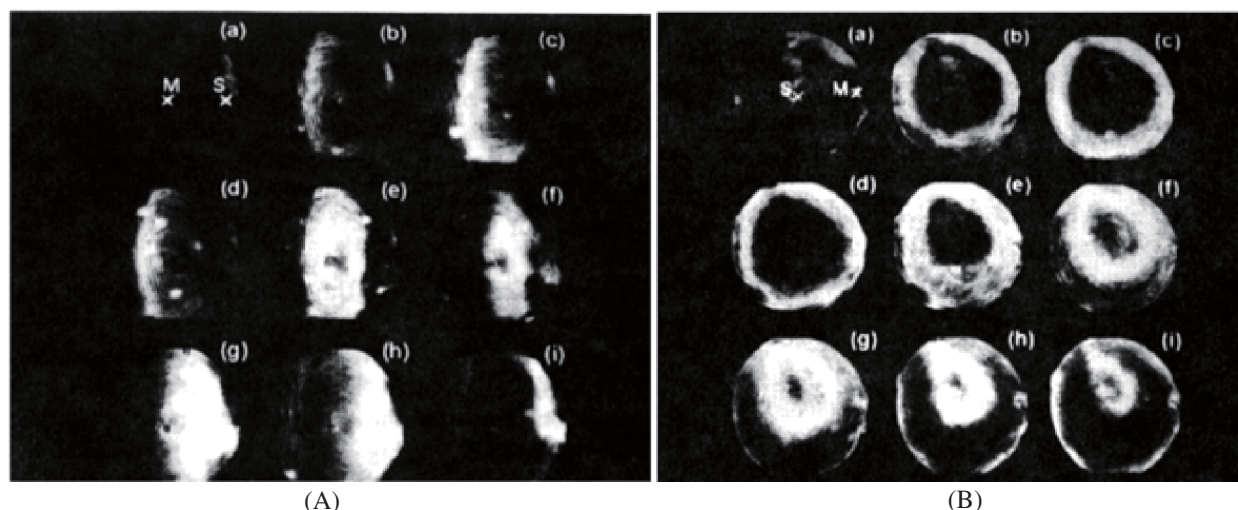
Fig. 18. Global views of the oscillatory flow in the systems with the spiral centers (at point S) near the right boundary in (A) and in the middle of the dish in (B). White bands (A) and white circular regions (B) show the flow waves, which propagate to the center of spiral waves. The images were obtained by background subtraction, smoothing, and contrast enhancement. The time delay between frames was 8.4 s. The points of flow measurement were located in points (M) (from Matthiessen and Müller (1995)).
