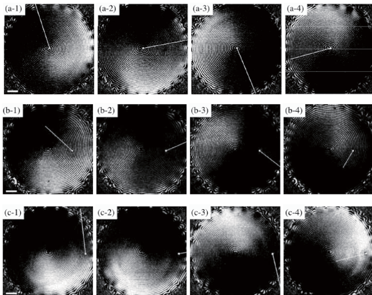
Fig. 22. Time sequences of a spiral flow wave with indication of the direction of surface flow (Mahara et al. , 2009). Pattern contrasts are emphasized so that only the flow wave pattern appears as a brighter area. The white dots in the respective pictures show observation points of the surface flow. The white lines indicate the direction of flow at the observation points; (a) r = 0 mm, (b) r = 33 mm, and (c) r = 66 mm, where r is the distance between the particular observation points and the chemical spiral center. The time interval is about 8 s. Scale bar in (a-1), (b-1), and (c-1): 10 mm.
