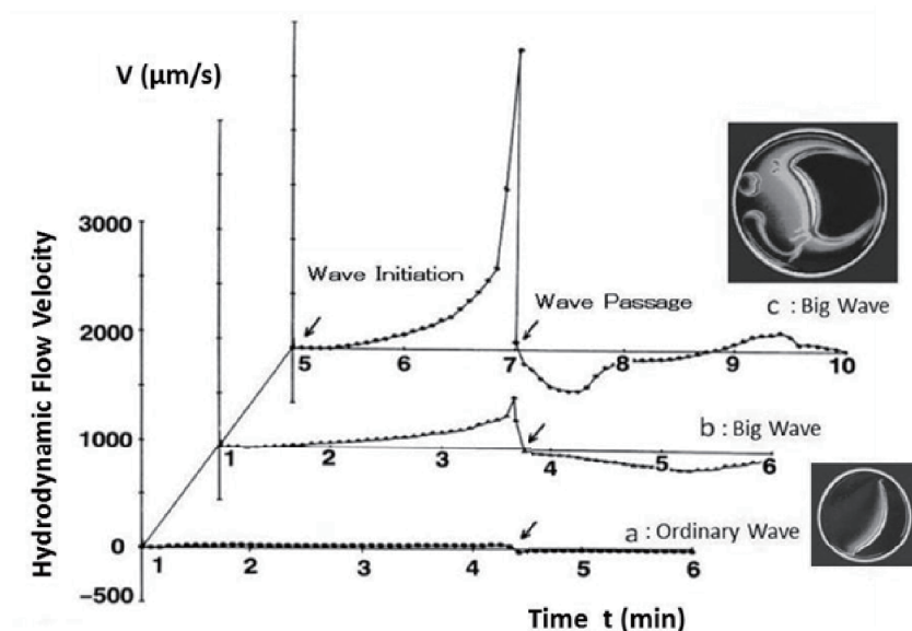
Fig. 11. Temporal traces of convective flow velocities induced by the ordinary chemical wave (a) and by the big waves (b, c) (Miike et al. , 1993).
