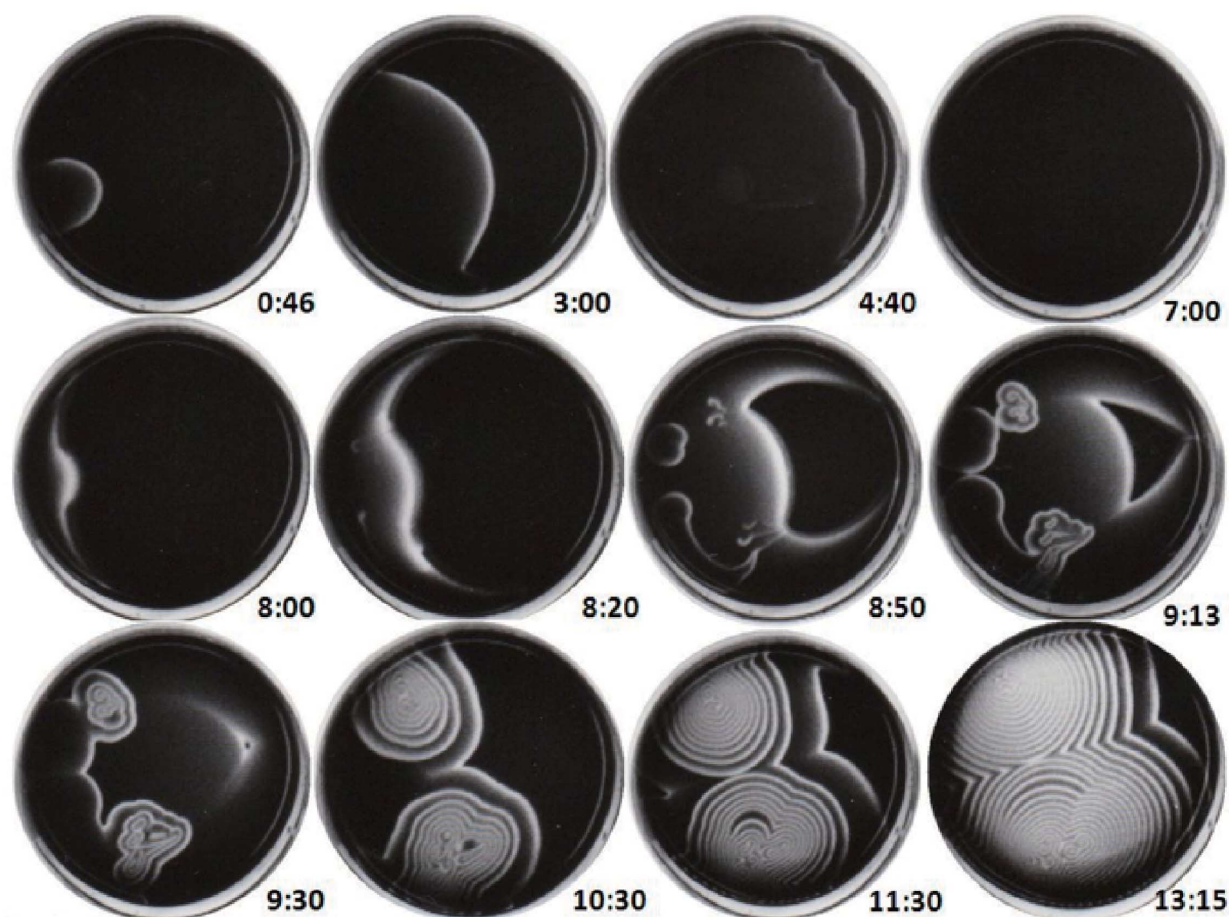
Fig. 1. Successive pattern dynamics coupled with chemically driven convections in a thin solution layer (depth 0.85 mm) of the BZ-reaction (Miike et al. , 1992).
