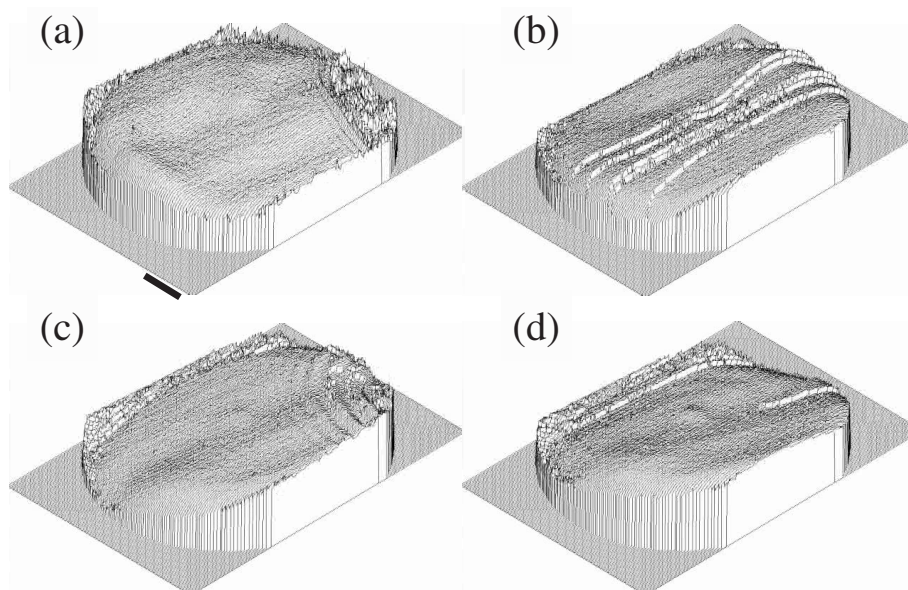
Fig. 23. Time series of analyzed surface deformation. The observation area is a circular region with a radius of 60 mm. The time interval between the 3D-plots is about 7.5 s. Scale bar in (a) is 10 mm (Mahara et al. , 2009).
