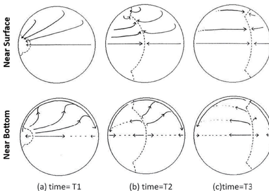
Fig. 12. Estimated horizontal flow structures based on repeated velocity measurement at many points of the Petri dish (Hashimoto et al. , 1991). Apparently, the single chemical wave propagation is accompanied by a propagating flow structure with a strong peripheral current near the bottom of the circular dish. The current is related to a larger propagation velocity of the big wave at the periphery of the dish (see Fig. 9).
