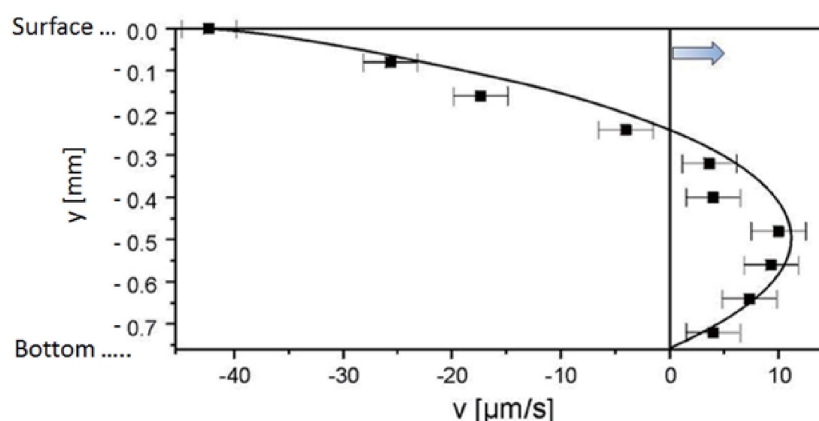
Fig. 14. Comparison between experiments (rectangles with error bar) and simulation (solid curve) for the velocity profile v(y) of convection induced by a single chemical wave. The grayish large arrow indicates the propagation direction of the chemical wave (Matthiessen et al. , 1996).
