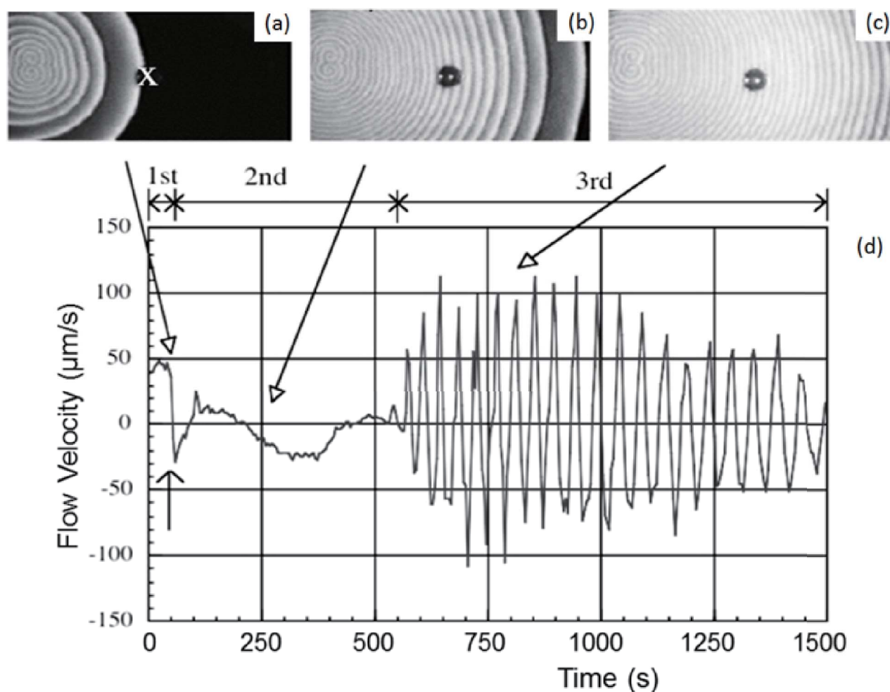
Fig. 15. Development of chemical spiral waves ((a) to (c): one spiral pair (OSP)) and temporal evolution of the flow velocity (d) measured near the surface of a BZ-solution layer at the center of a Petri dish (Sakurai et al. , 1997b). (a), (b), and (c) are image samples observed at about t = 50 , 250, and 800 s, respectively. The position marked x in (a) indicates the location of measurements of flow velocity. The oscillatory flow started in the third stage after t = 550 s and continued for more than 1000 s.
