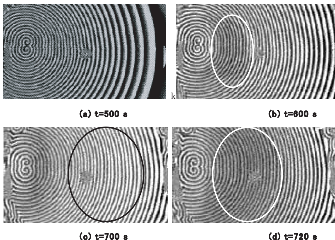
Fig. 19. Initiation and propagation of flow waves induced in a thin BZ-solution layer after exciting a chemical spiral wave train (Miike et al. , 2010). (a) Before initiation of flow waves, (b) just after flow wave initiation. Images (c) and (d) show the phase of flow waves with a brighter profile (c) and a darker one (d). The flow waves were initiated at the right boundary of the dish and propagated toward the core of the spiral waves. The white ellipse contains the darker profile area of the flow waves, while the black ellipse shows the brighter one, which corresponds to the white band in Fig. 18(A).
