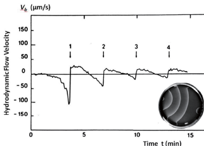
Fig. 8. Time trace of the flow velocity V_b measured near the bottom of the solution at the middle of the dish. Discrete chemical waves (numbered 1, 2, 3, and 4) of the “target pattern” are induced spontaneously by triggering a single circular wave at the left end of the dish (see the picture) (Miike et al. , 1988; Miike and Müller, 1990; Miike and Sakurai, 2003). The direction of chemical wave propagation coincides with that of negative flow velocity. The flow velocity measured near the surface V_s has a larger amplitude and opposite direction.
