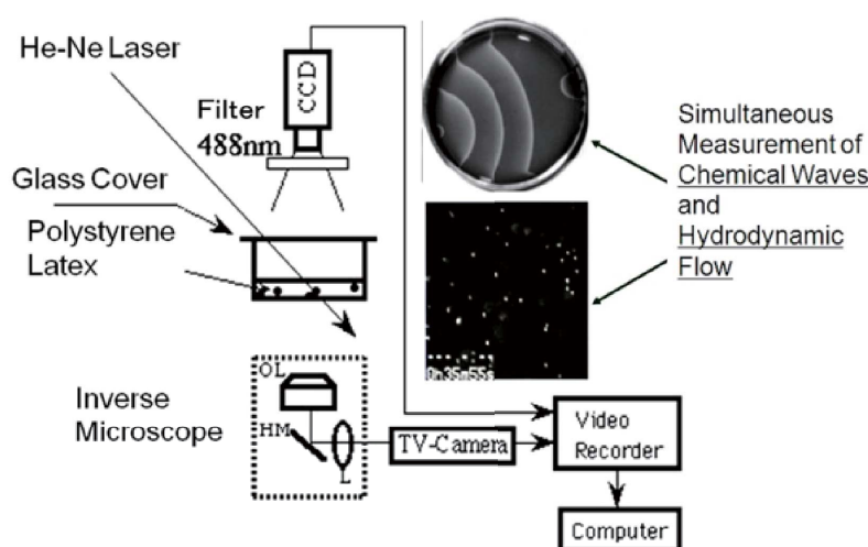
Fig. 3. Schematic diagram of the microscope video imaging system (Müller et al. , 1985; Miike et al. , 1992). Simultaneous measurement of chemical activity and hydrodynamic motion was realized.
