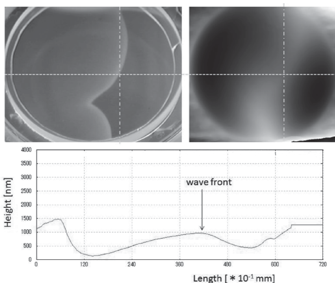
Fig. 26. Deformation of an air-liquid interface induced by CDC in a thin solution layer of the BZ-reaction (Okada et al. , 2007). The upper left figure shows the propagation of circular waves in a Petri dish, the upper right one a result of surface deformation analysis from a fringe pattern of a Fizeau interferometer. The lower figure shows a cross section of the surface deformation along the broken line in the upper figures.
