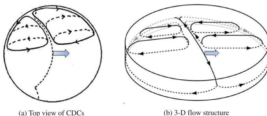
Fig. 13. A schematic model for the three-dimensional flow structure of CDCs induced by a single chemical wave (see Fig. 6). The broken line in (a) shows the front of chemical activity, and grayish large arrows show its propagating direction. Solid lines with an arrow in (b) indicate the hydrodynamic flows near the surface of the BZ-solution. Dashed lines with arrows show the flows near the bottom of the solution (Hashimoto et al. , 1991).
