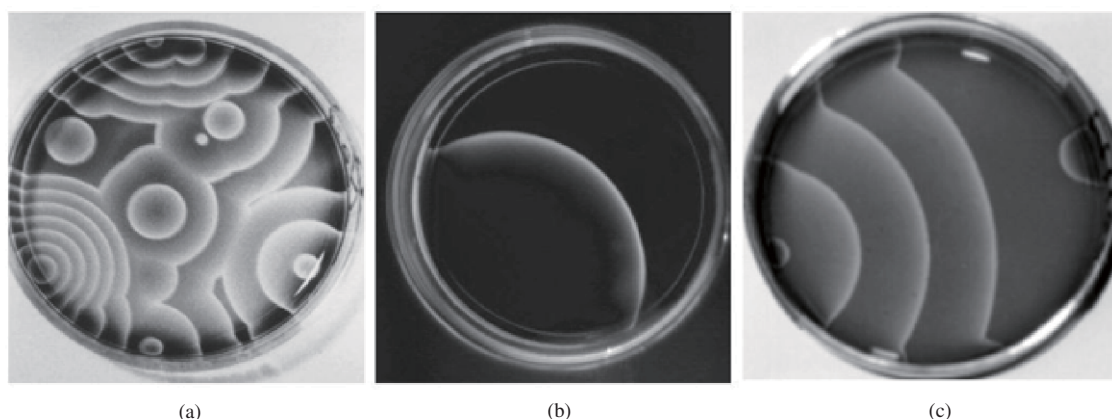
Fig. 2. (a) Target patterns of chemical activity under uncontrolled condition, (b) and (c) single circular wave and a target pattern, respectively, under well controlled condition (Castets et al. , 1990; Sakurai et al. , 1997b). Under such a condition, except for the triggered wave any spontaneous initiation of chemical waves is almost suppressed during the triggered wave propagation (see (b)) in the Petri dish (diameter 6.8 cm).
