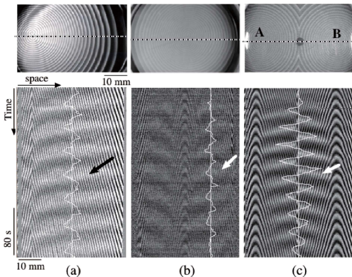
Fig. 20. Space-time plot of chemical activity modified by oscillatory flow induced in three types of spiral systems (Sakurai et al. , 2004). The white lines superimposed on the space-time plot correspond to the flow velocity development in Fig. 15. The line plotted in (b) is the velocity measured between the spiral center and the boundary of petri dish. (a) OSP1 system. (b) OSP2 system. (c) TSPs system.
