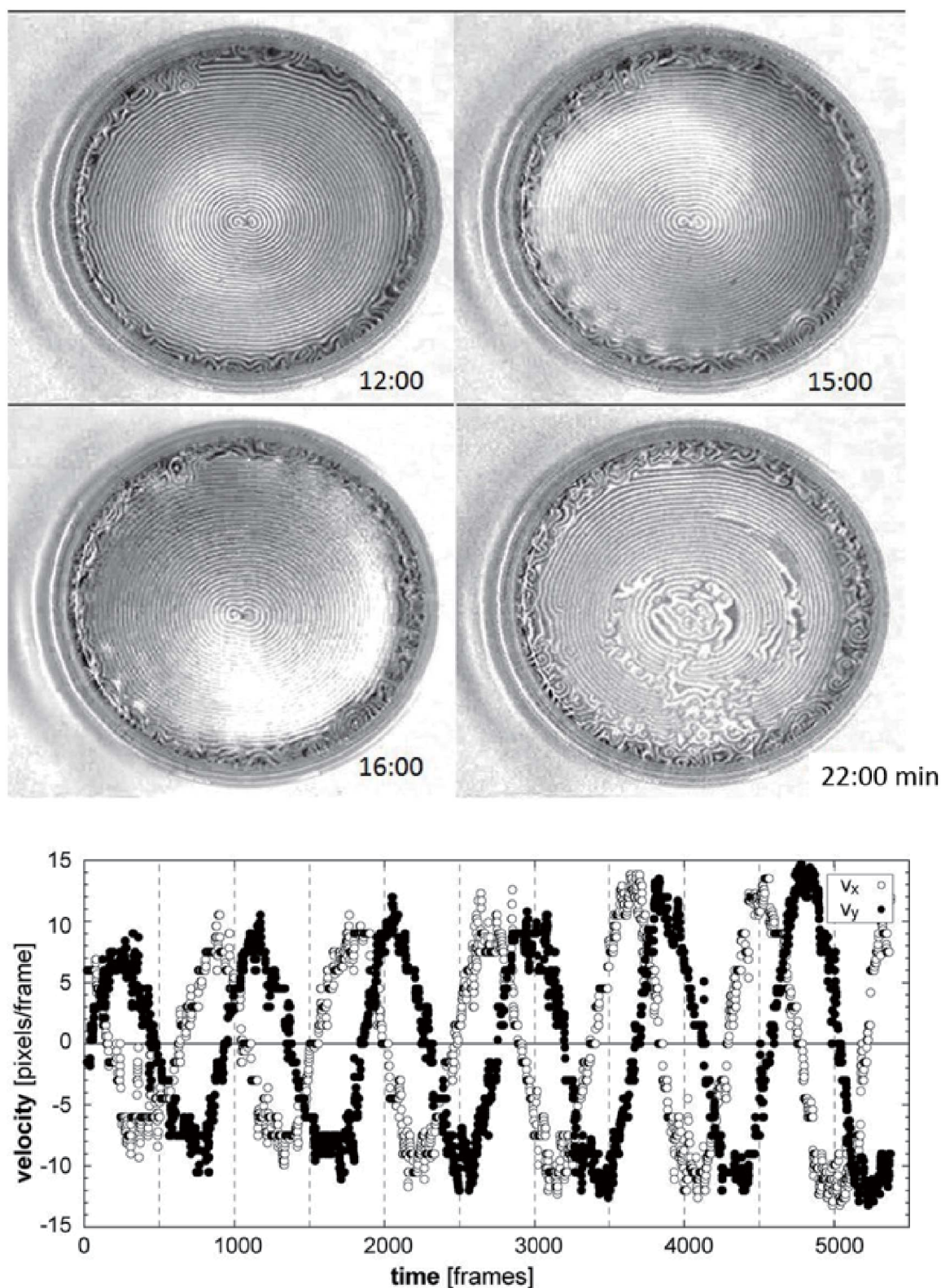
Fig. 21. Time series of a spiral flow wave (top 4 pictures). A chemical spiral pair was triggered at the middle of the dish ( t = 0 : 00 min). Other than in Fig. 20, the spiral-shaped flow wave started from the chemical spiral pair ( t = 12 : 00 min) and propagated in outward direction. A rotating surface flow was accompanied by the flow wave. The surface flow did not stabilize to a motionless state but grew in amplitude (see the bottom figure sampled by 30 Hz: 1 s = 30 frames) until the system is self-collapsed ( t = 22 : 00 min) (Miike et al. , 2010). The top pictures are obtained by image processing, which is based on a new pixel-based temporal brightness enhancement (Otaka et al. , 2013).
