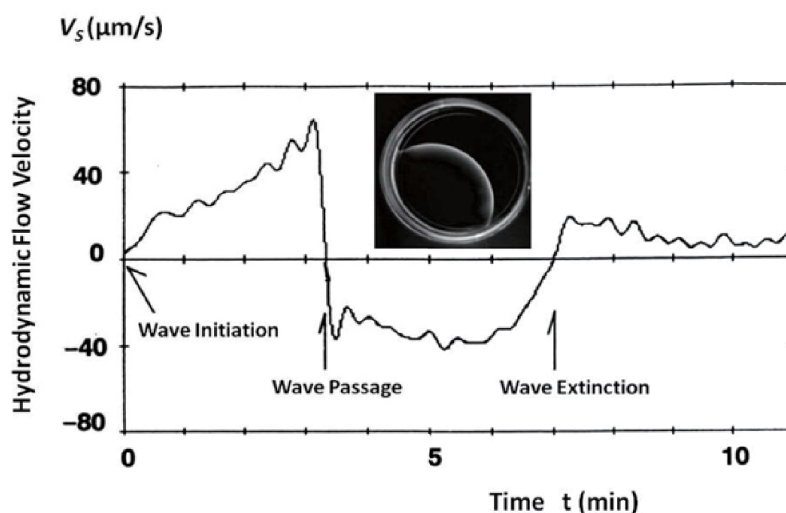
Fig. 7. Temporal trace of convective flows associated with single circular wave propagation. The chemical wave propagation causes a gradual increase of hydrodynamic velocity observed at the middle of the Petri dish (Miike et al. , 1988; Miike and Sakurai, 2003).
