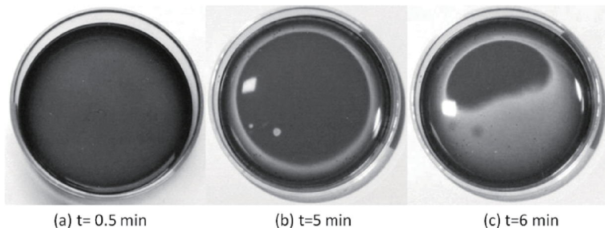
Fig. 4. Relaxation process to a well reduced state of the BZ solution. After the reduction of the solution, a “kinematic wave” propagated with high speed. There is almost no spontaneous induction of chemical waves during the reduction stage (0–5 min).
