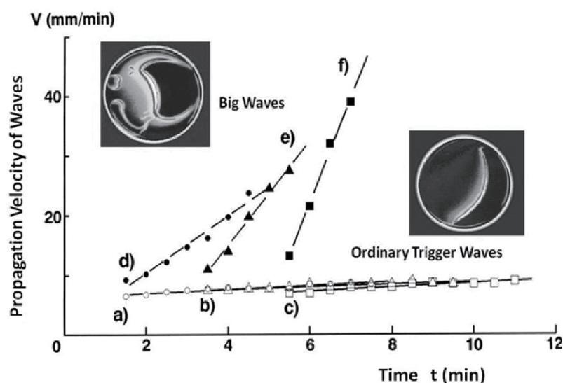
Fig. 10. Time evolution of propagation velocity of chemical waves (Miike et al. , 1993). a) \circ , b) \triangle , and c) \square ordinary waves are triggered at t = 1, 3 , and 5 min after mixing the BZ-solution, respectively. d) \bullet , e) \blacktriangle , and f) \blacksquare : big waves are triggered at t = 1, 3 , and 5 min, respectively.
